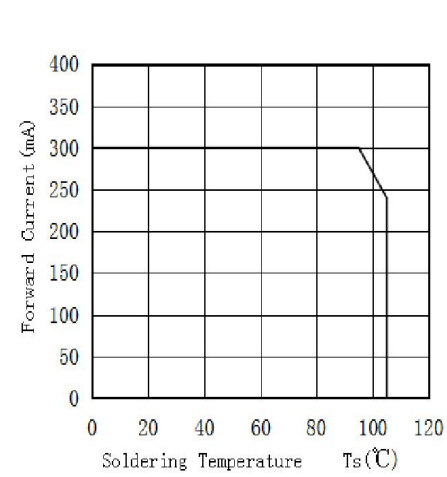
Soldering Temperature VS Allowable Forward Current 焊盘温度与允许温度电流特性
